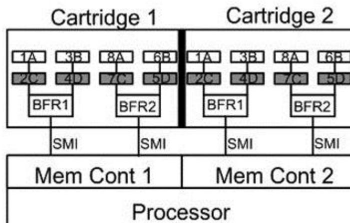
Figure 1 Processor/Memory interconnect
