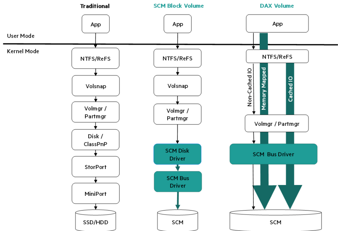
Figure 2. I/O stack comparisons
