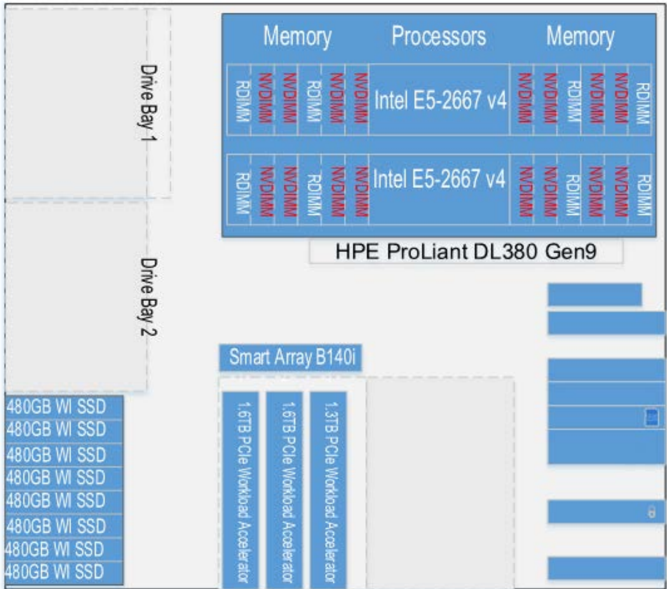
Figure 3. Diagram of memory and disk layout for HPE ProLiant DL380 Gen9 server
