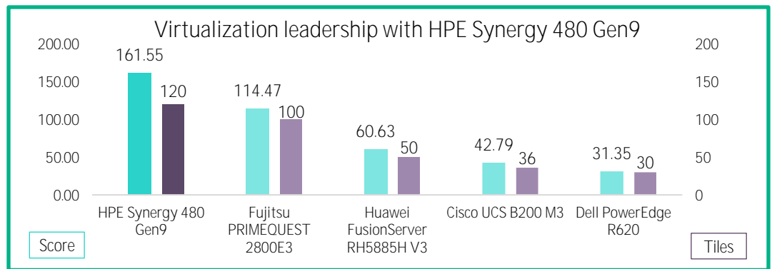
Figure 1. HPE world record result compared to the top result from four other vendors on the VMmark 2.x benchmark.
