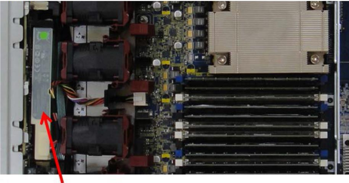
Remove megacell
